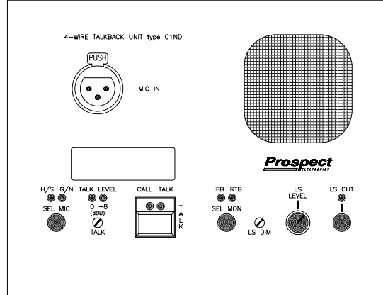
C1ND TOP PANEL
